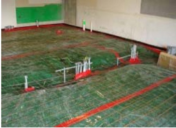
Under-slab Vapor Barrier
